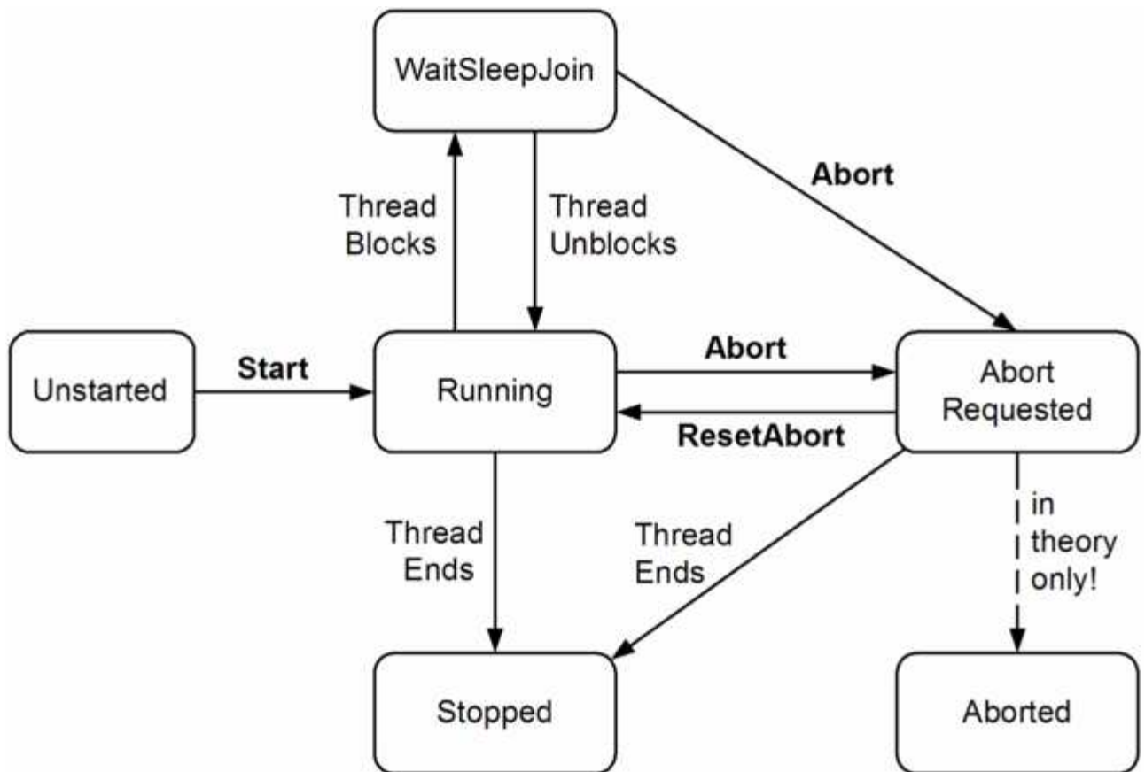
Figure 1: Thread State Diagram
